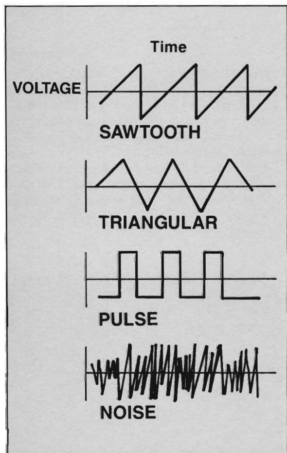
Figure 6.9. Sawtooth, triangular, pulse, and noise SID waveforms.
